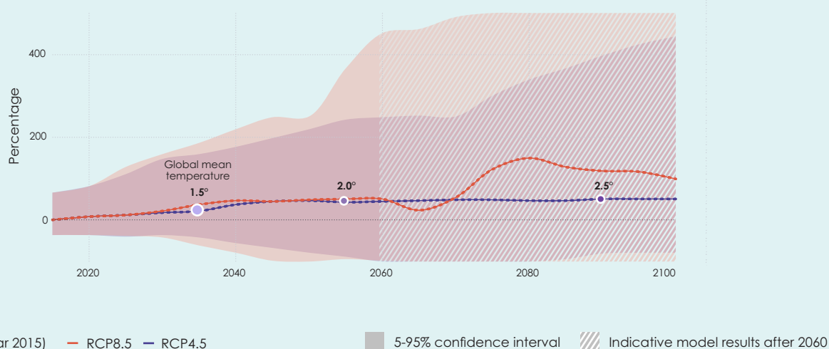
(a) Annual Expected Damage from River Floods in Percentage
